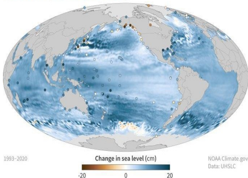
SEA LEVEL CHANGE (1993-2020)
